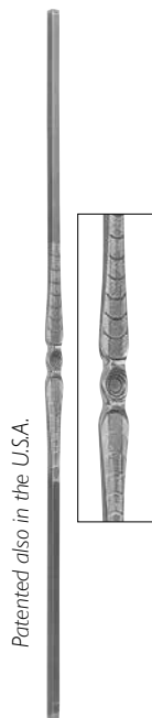
Art. 1702/2/ALL Mtl 9/16" sq. H 39 3/8" Wt. 3.4 lbs.
