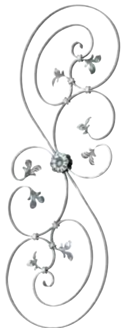
Art. 1670/1/ALL Mtl 1/2" x 1/4" W 14 3/16" H 39 1/2" Wt. 2.78 lbs.
