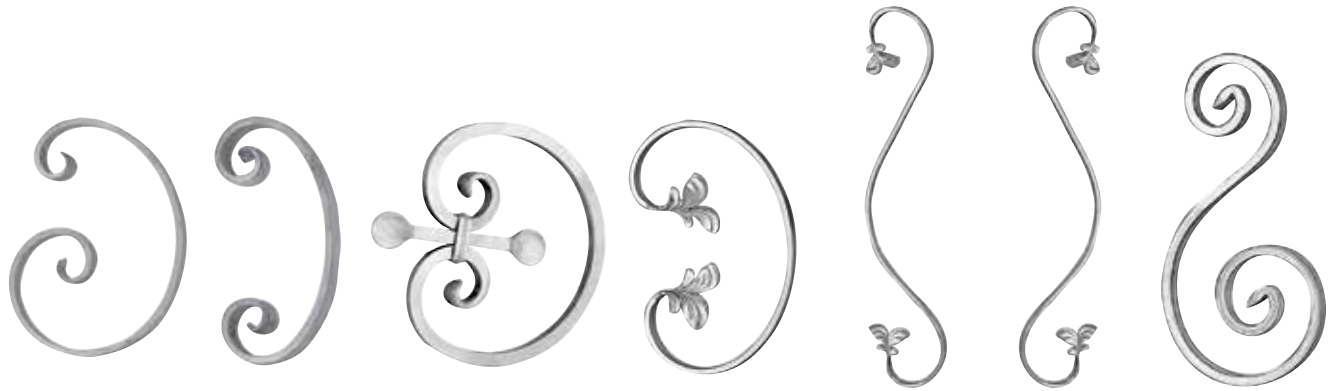
Art. 1437/18 Mtl 3/4" x 1/4" W 5 3/4" H 8 1/16" Wt. 0.1 lb. Art. 1437/19 Mtl 3/4" x 1/4" W 3 1/2" H 7 9/32" Wt. 0.1 lb. Art. 1867/4 9/16" sq. W 10 1/32" H 10 5/8" Wt. 1.3 lbs. Art. 770/1 Mtl 3/4" x 1/4" W 6 5/16" H 9 7/8" Wt. 0.3 lb. Art. 770/2 Mtl 1/2" x 1/4" W 4 3/8" H 20" Wt. 0.37 lb. Art. 770/2/DX Mtl 1/2" x 1/4" W 4 3/8" H 20" Wt. 0.37 lb. Art. 770/3 Mtl 1/2" x 1/4" W 4 3/4" H 8 11/16" Wt. 0.3 lb.
